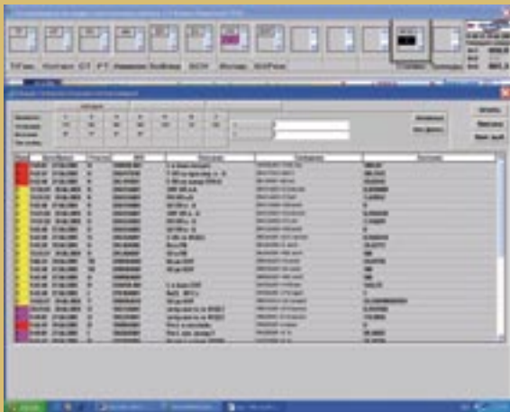
An Alarm Summary Screen at Permskaya Gres Power Plant
