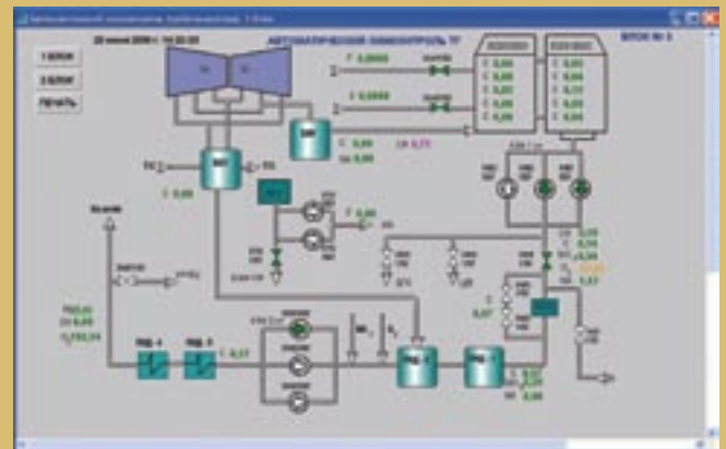
A Power Plant Control Screen
